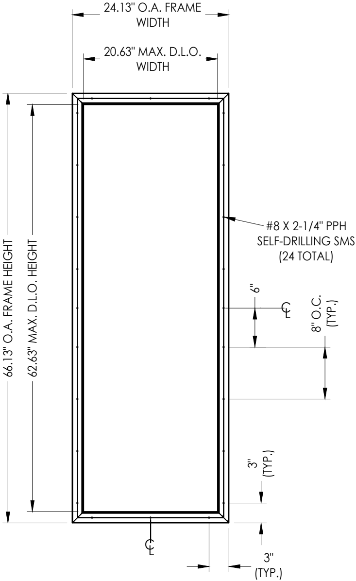
ODL 6'-8" IMPACT PVC LITE FRAME "KEystone"
