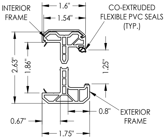
2B ODL KEYSTONE PVC LITE FRAME 1-1/4" GLAZING
