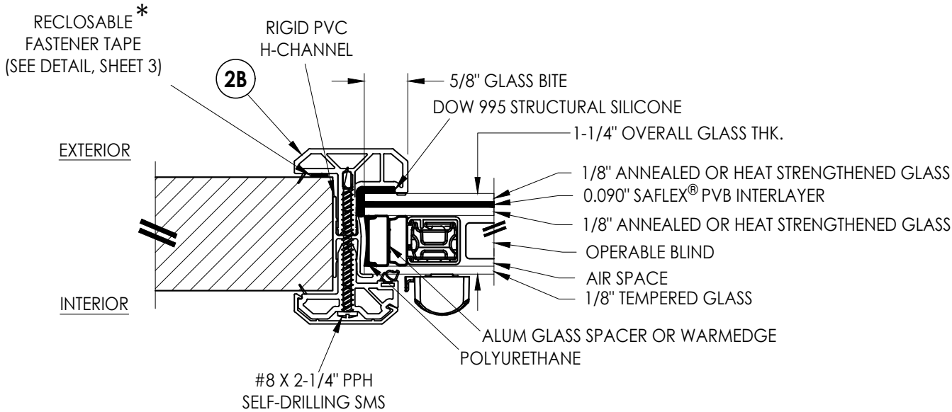
G4 GLAZING DETAIL ALUM SPACER w/ OPERABLE BLIND
