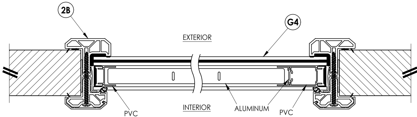
2 HORIZONTAL CROSS SECTION 4 WARMEDGE OPERABLE BLIND
