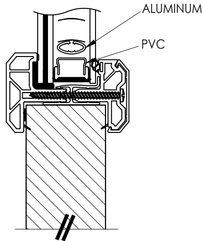
1 VERTICAL CROSS SECTION 4 WARMEDGE OPERABLE BLIND
