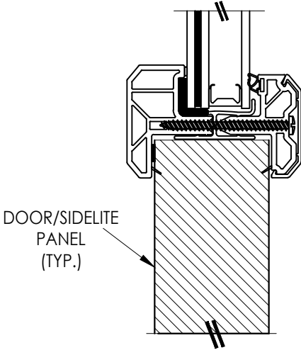
1 2 VERTICAL CROSS SECTION
