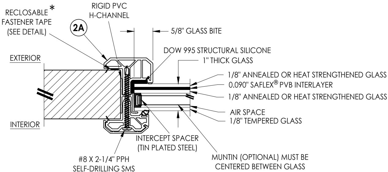
G3 GLAZING DETAIL INTERCEPT SPACER w/ OPTIONAL MUNTIN
